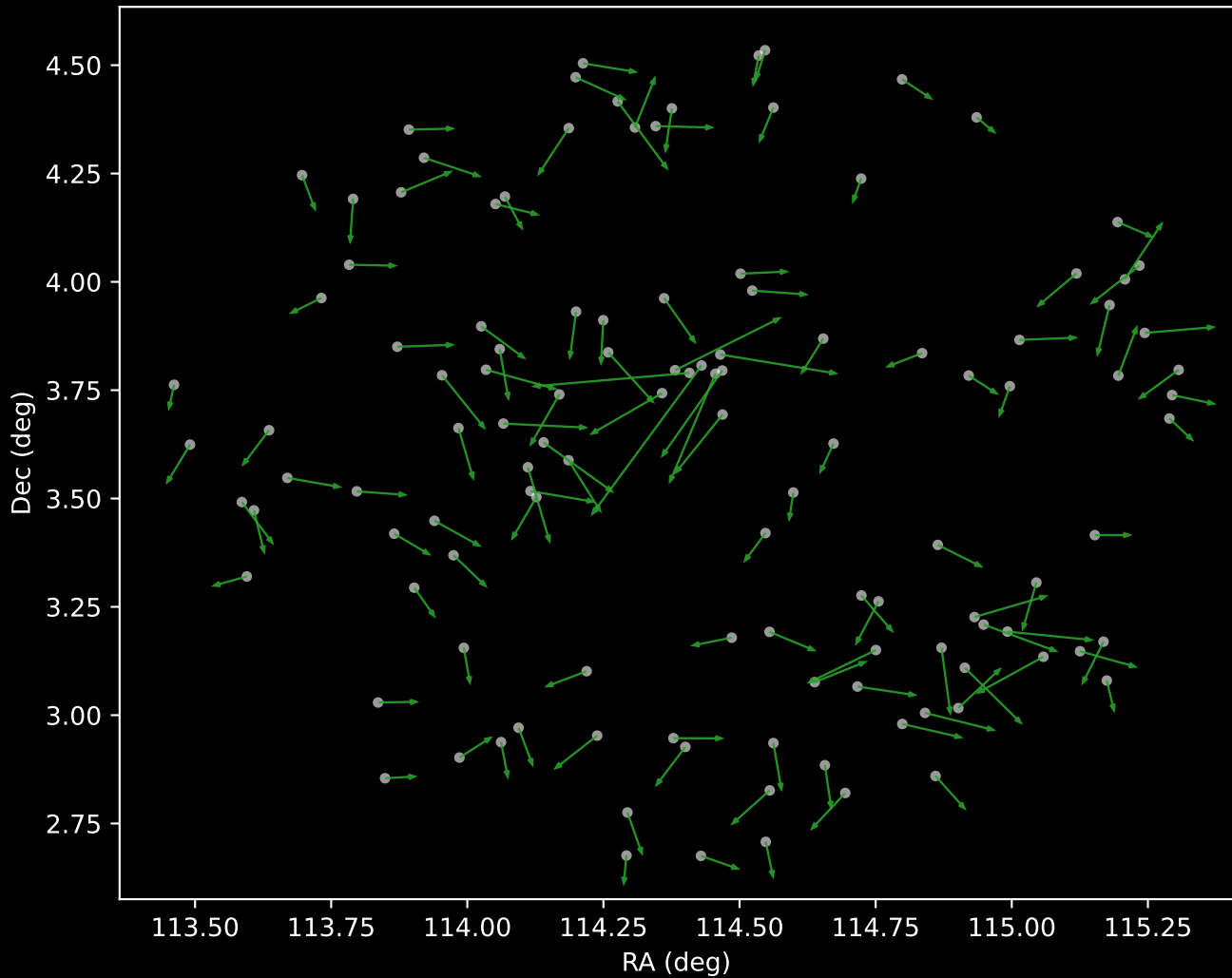
APOGEE DR17 Cluster 4 Proper Motion Vectors (n=120)
