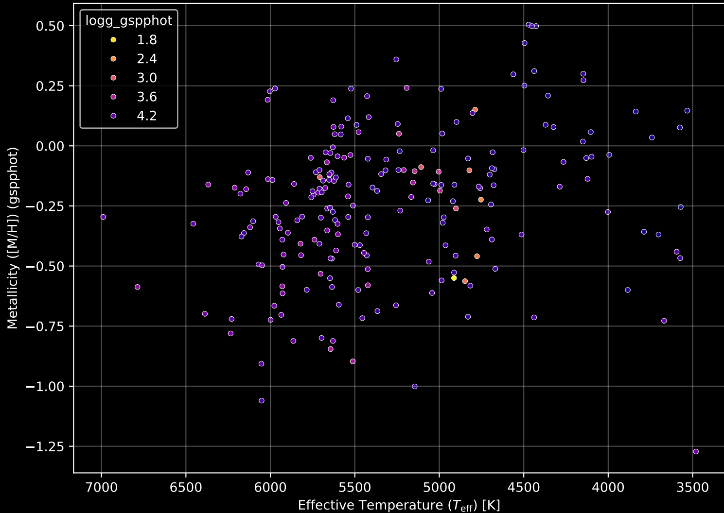
APOGEE DR17 Field: [126-59-O] Stellar Population Parameters (n= 214)
