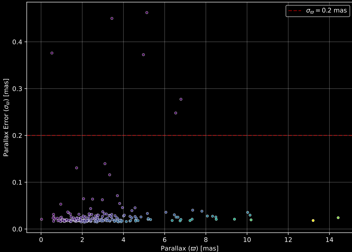
APOGEE DR17 Field: [126-59-O] Parallax Quality (n= 214)
