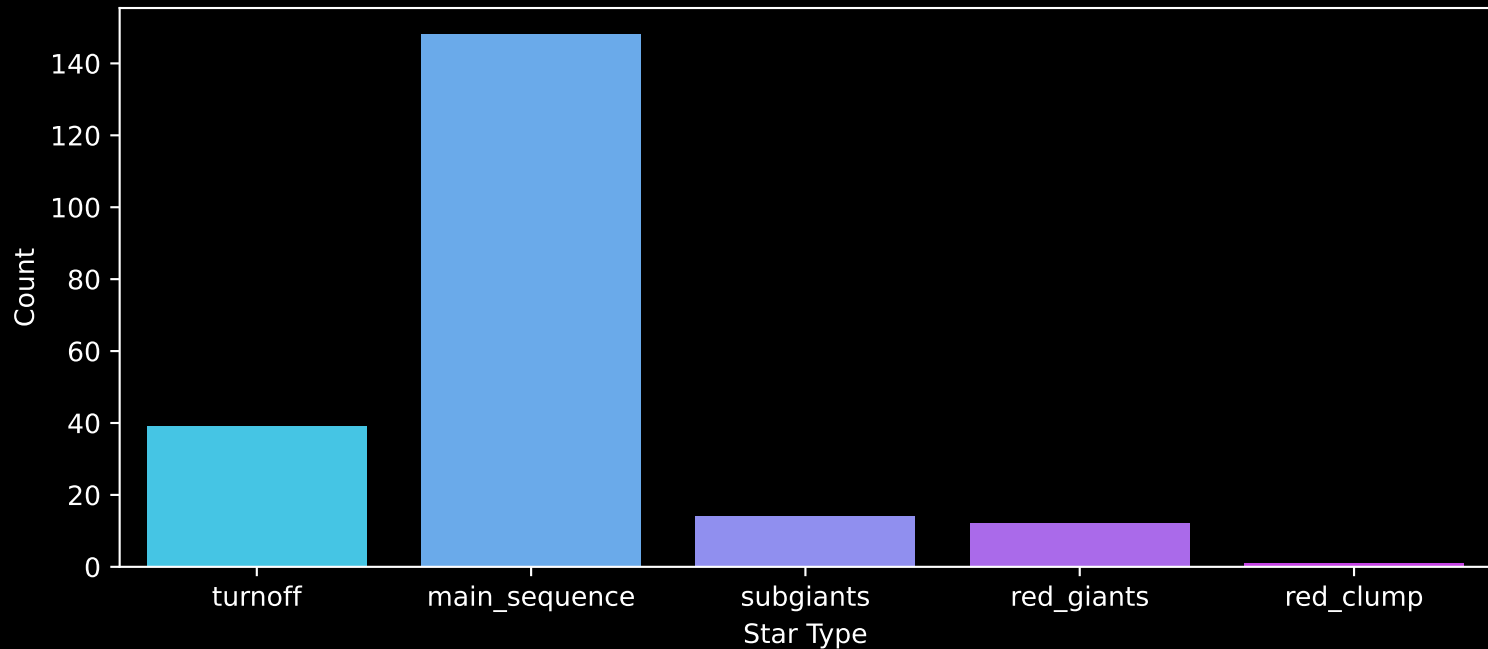
APOGEE DR17 Field: [126-59-O] Count plot of Star Type
