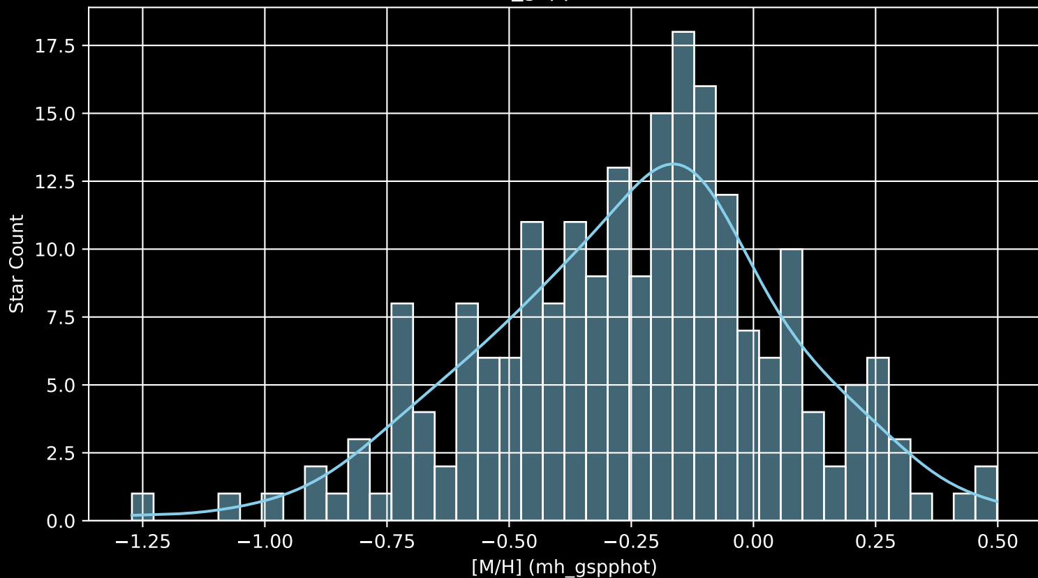
APOGEE DR17 Field: [126-59-O [M/H] (mh_gspphot) (n= 213)
