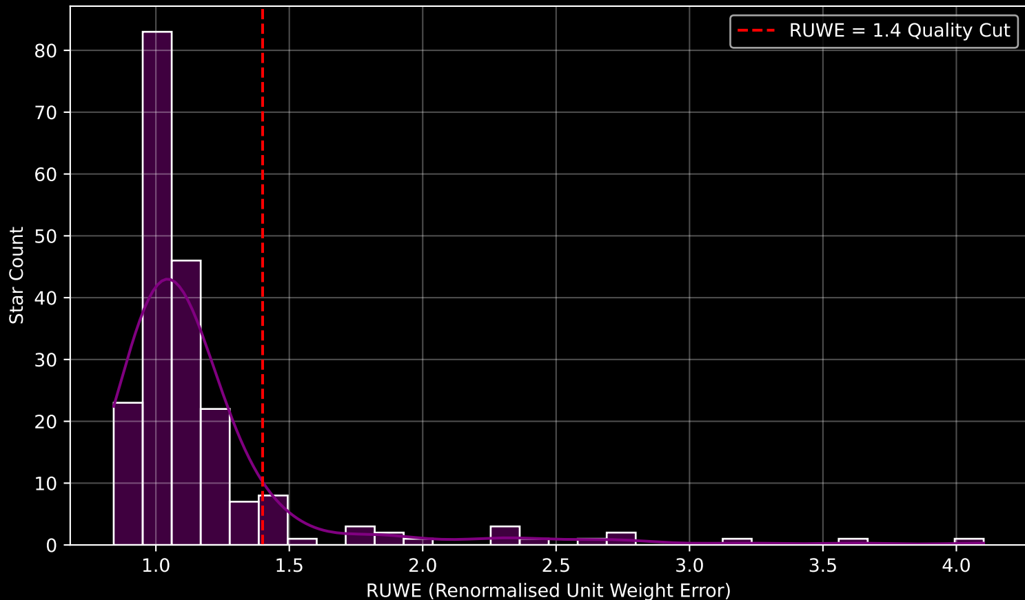
GAPOGEE DR17 Field [126-59-O] RUWE Distribution (n= 206)
